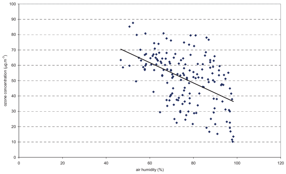
Fig. 10. Correlation of ozone concentration – moisture, 1998.
