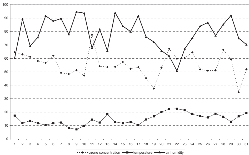
Fig. 13. Relation of ozone concentration to moisture and temperature, July 1998.
