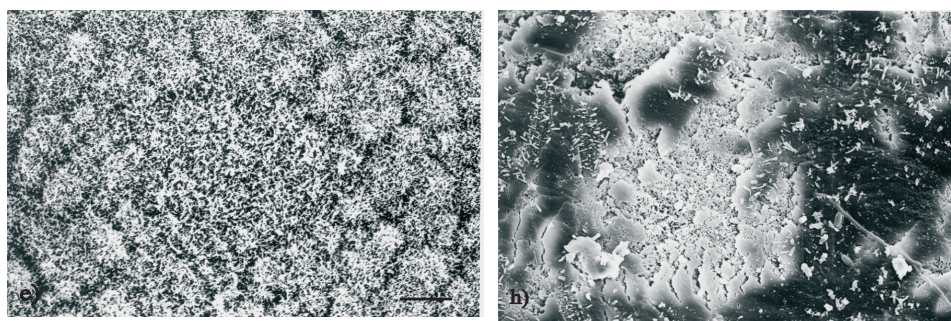
Fig. 2. Microstructure epicuticular waxes in epistomatal area A. alba M i l l. Note: classes: e) classification class I, h) classification class IV, abscisa represents 10 µm.
