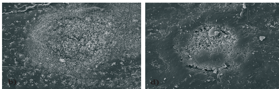
Fig. 1. Microstructure epicuticular waxes in epistomatal area P. abies K a r s t. Note: classes: b) classification class I , d) classification class IV, abscisa represents 20µm
