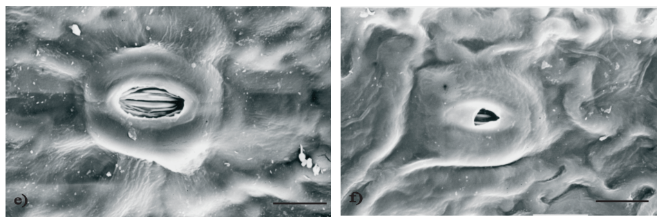
Fig. 3. Microstructure epicuticular waxes in epistomatal area of F. sylvatica L. Note: e) classification class I; f) classification class III, abscissa represents 10 µm
