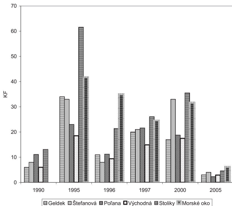
Fig. 1. Exceedance of element concentration ( K_F ) in mosses in the years 1990–2005. Note: K_F for Cd, Fe, Hg, Pb and Zn
