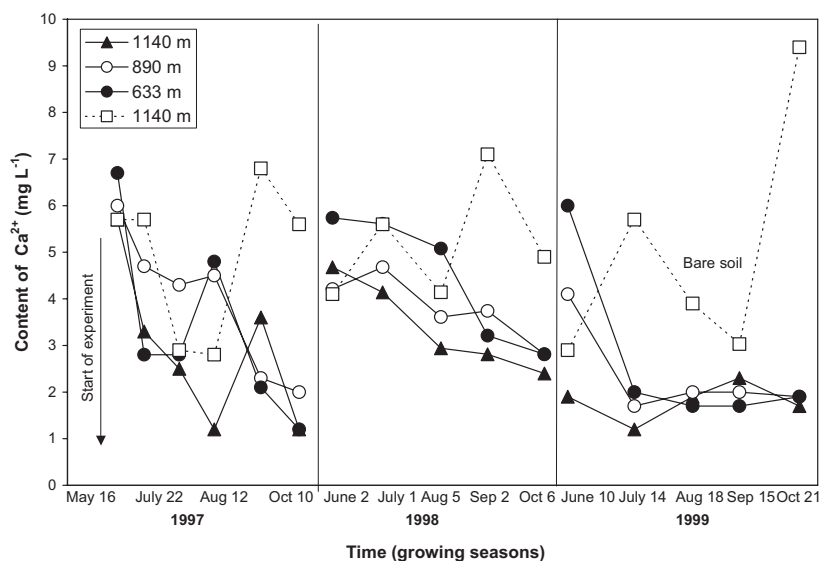
Fig. 3. Changes in concentration of Ca 2+ of lysimetric water leached from old Calamagrostis villosa swards on different sites and from bare forest soil (1140 m a.s.l. – Malý Smrk Mt.) during 1997, 1998 and 1999 growing seasons. Mean values are shown.
